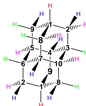
Fig. (6). A. Numbering of adamantane carbon atoms. B. Numbering of diamondane carbon atoms.
