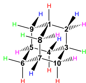
Fig. (6). A. Numbering of adamantane carbon atoms. B. Numbering of diamondane carbon atoms.
